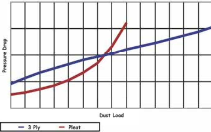
RESISTANCE vs. DUST LOADING
